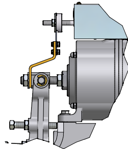
90 BRAKE DETAIL A
