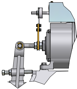
100 & 110 BRAKE DETAIL A
