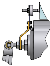
120 BRAKE DETAIL A
