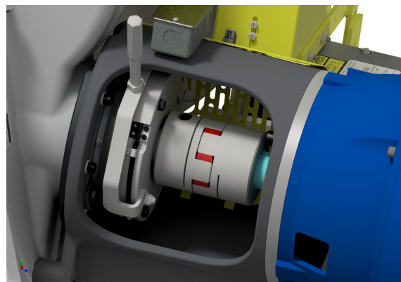
Flexible Motor Coupling Mating to Flexible Worm Shaft Coupling
