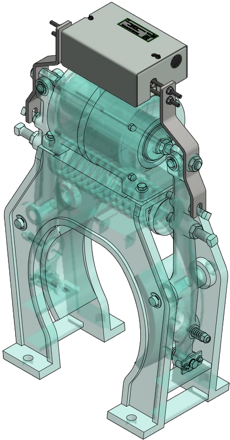
MONITOR KIT SHOWN INSTALLED ON #90 BRAKE. #80, 81, 85, 86, & 91 SIMILAR
