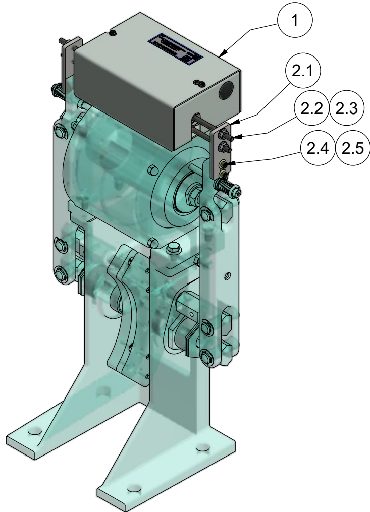
MONITOR KIT SHOWN INSTALLED ON BRAKE w/OLD STYLE BRAKE ARMS. ITEM 2.6 NOT USED. #102 BRAKE SHOWN, #112 BRAKE SIMILAR
