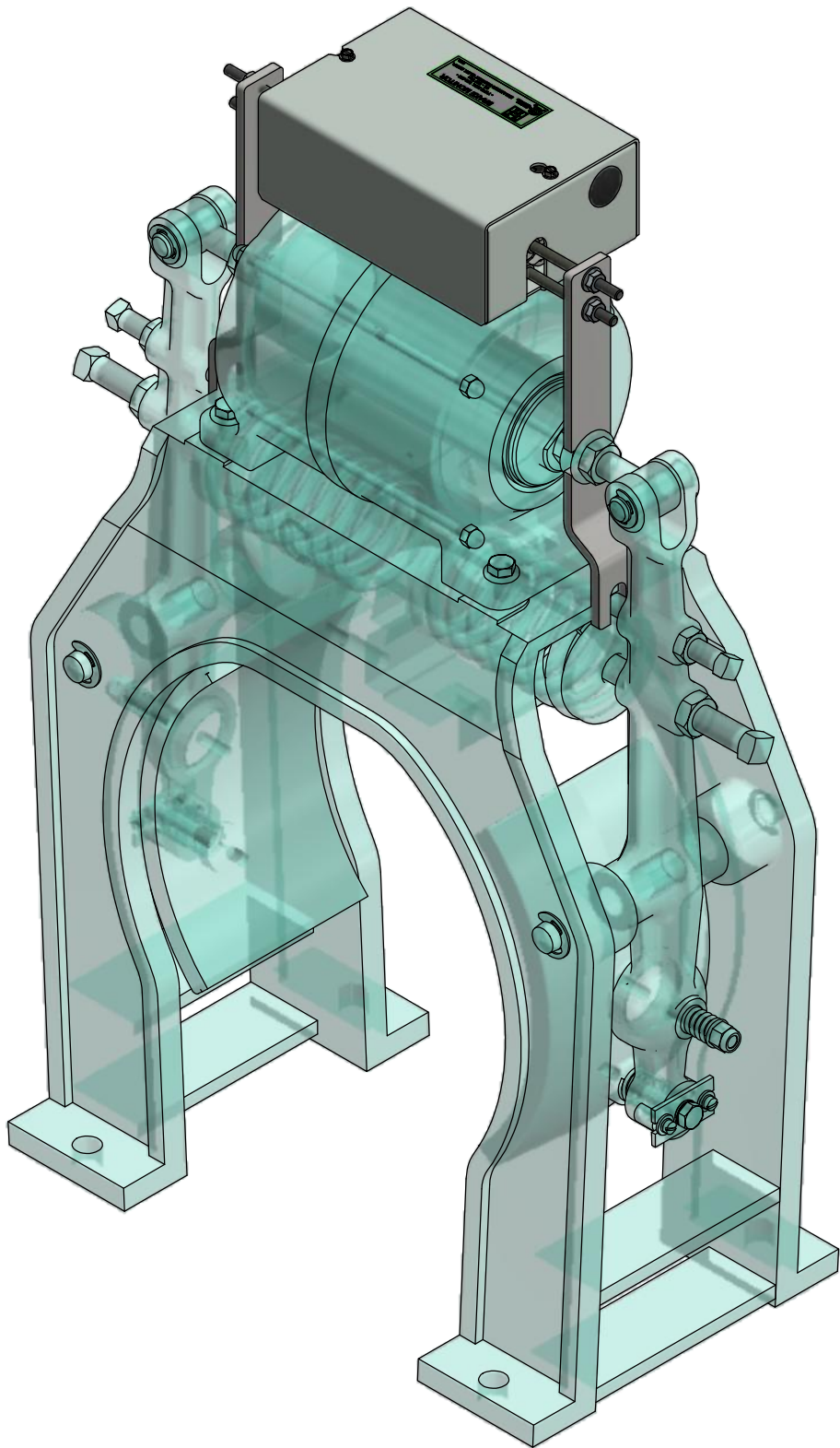
MONITOR KIT SHOWN INSTALLED ON #100 BRAKE. #95, 96, 101, 105, 106, 110, & 111 BRAKES SIMILAR.
