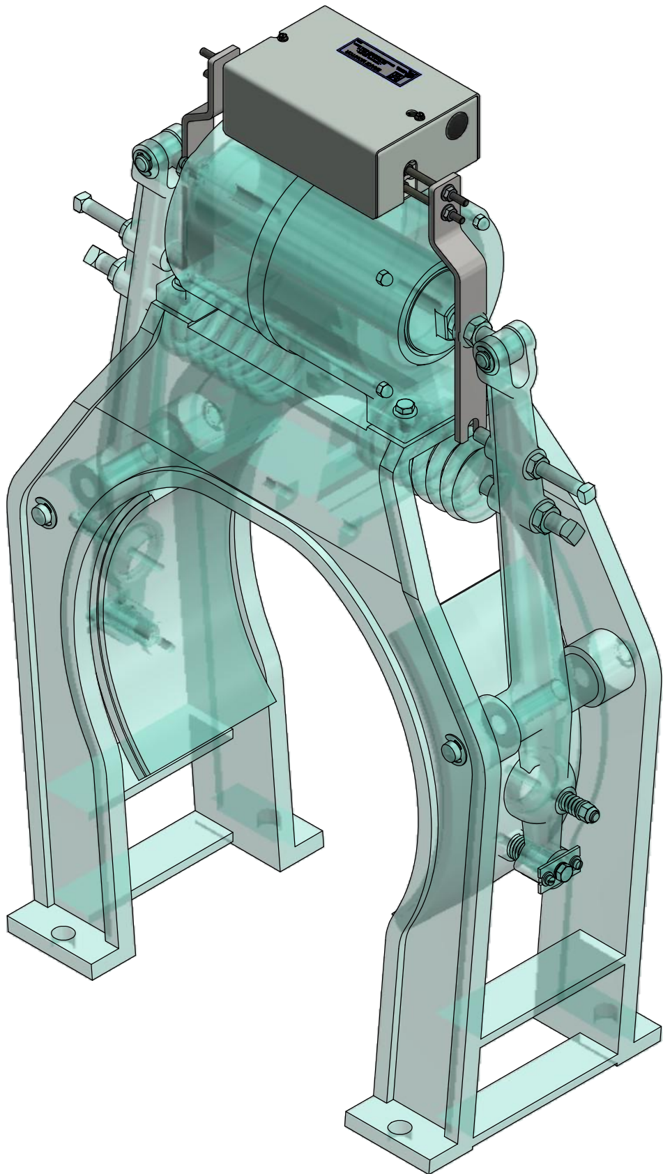
MONITOR KIT SHOWN INSTALLED ON #120 BRAKE. #115, 116, 121 & 125 BRAKES SIMILAR
