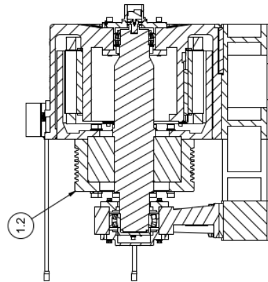
SECTION B-B SCALE 1:12
